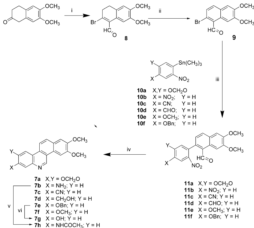
Scheme 1. (i) DMF, PBr 3 , CHCl 3 , reflux; (ii) DDQ, toluene, reflux; (iii) (CH 3 ) 3 SnSn(CH 3 ) 3 , Pd(PPh 3 ) 4 , THF, reflux; (iv) Zn, AcOH, reflux; (v) Ac 2 O, pyridine; (vi) H 2 , 45 psi, Ra–Ni, MeOH; EtOAc/THF.
